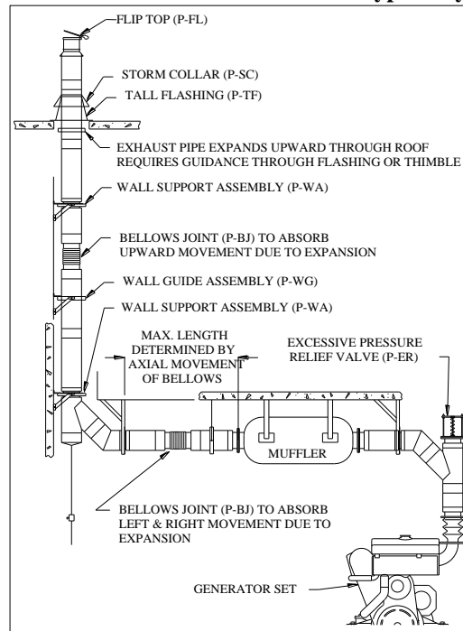
Fig. C-2 - Bellows Joints (P-BJ)
